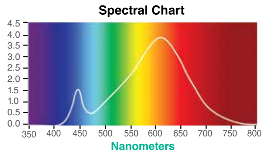
item# 1003859 UTOPIA LED 3W G25, CLEAR, WW
