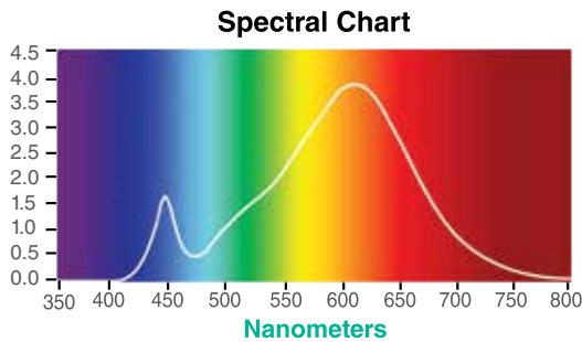
item# 1003863 UTOPIA LED 3W G16.5, CLEAR, WW
